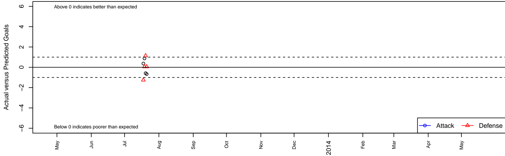
North Rockland Sting G99 Dots are actual minus expected GF (blue circles) and GA (red triangles). Blue line is smoothed change in attack strength. Red is smoothed change in defense strength.
